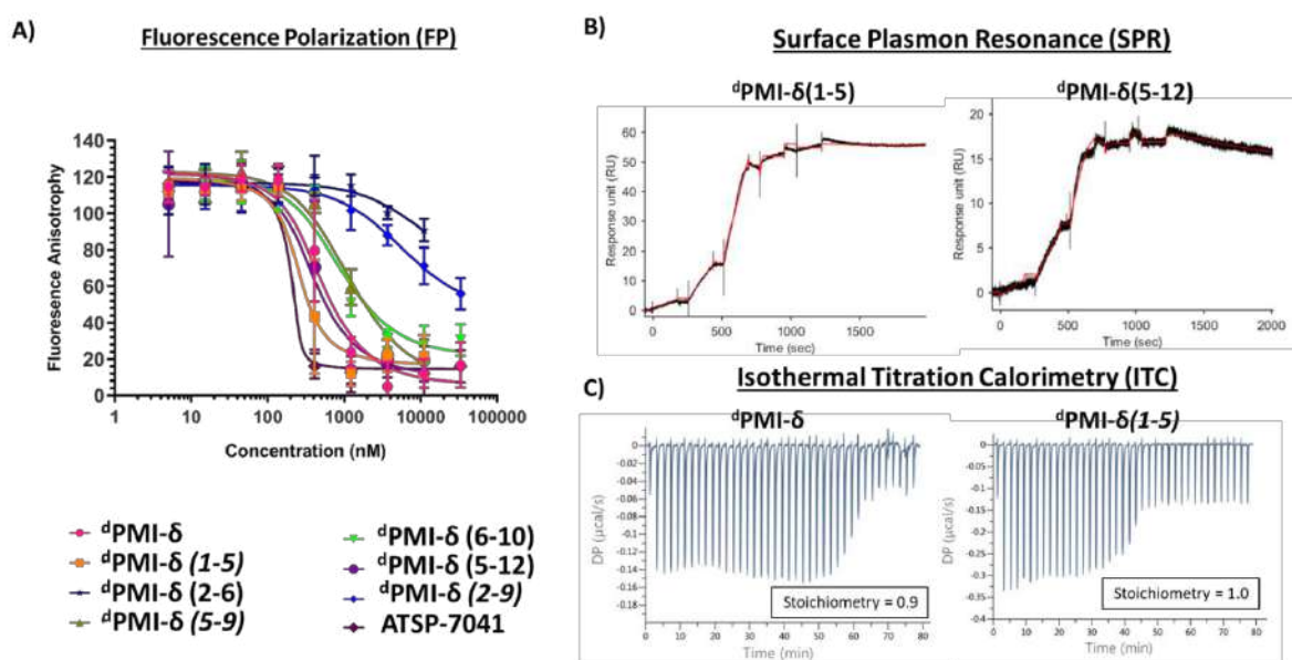
Figure 5: Binding activity of stapled ^d\text{PMI-}\delta peptides toward Mdm2 protein determined through various biophysical and biochemical methods. (A) Fluorescence polarization (FP) (0.001% Tween-20) binding analysis of linear, stapled ^d\text{PMI-}\delta and ATSP-7041 peptides and Mdm2 protein. Binding activity of peptides toward Mdm2 protein determined through (B) Surface Plasmon Resonance (SPR) and (C) Isothermal Titration Calorimetry (ITC).
