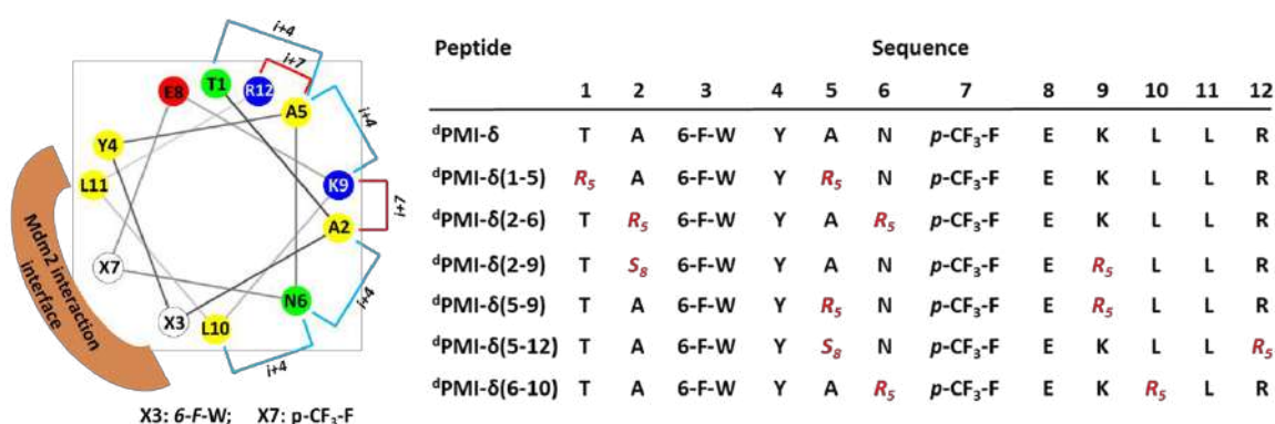
Figure 2: A helical wheel representation of the dPMI- \delta template sequence used for the design of stapled peptides. Residues that are linked through all hydrocarbon linkers i, i+4 and i, i+7 are highlighted in blue and red respectively. Sequences of the linear and stapled dPMI- \delta peptides are shown on the right.
