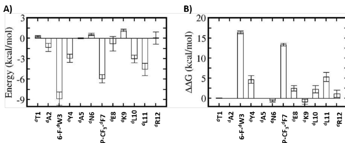
Figure 1: Energetic analysis of the MD simulations of the d PMI- \delta – Mdm2 complex. (A) Binding free energy contributions of the d PMI- \delta peptide residues. (B) Computational alanine (D- ala) scanning of d PMI- \delta peptide residues.
