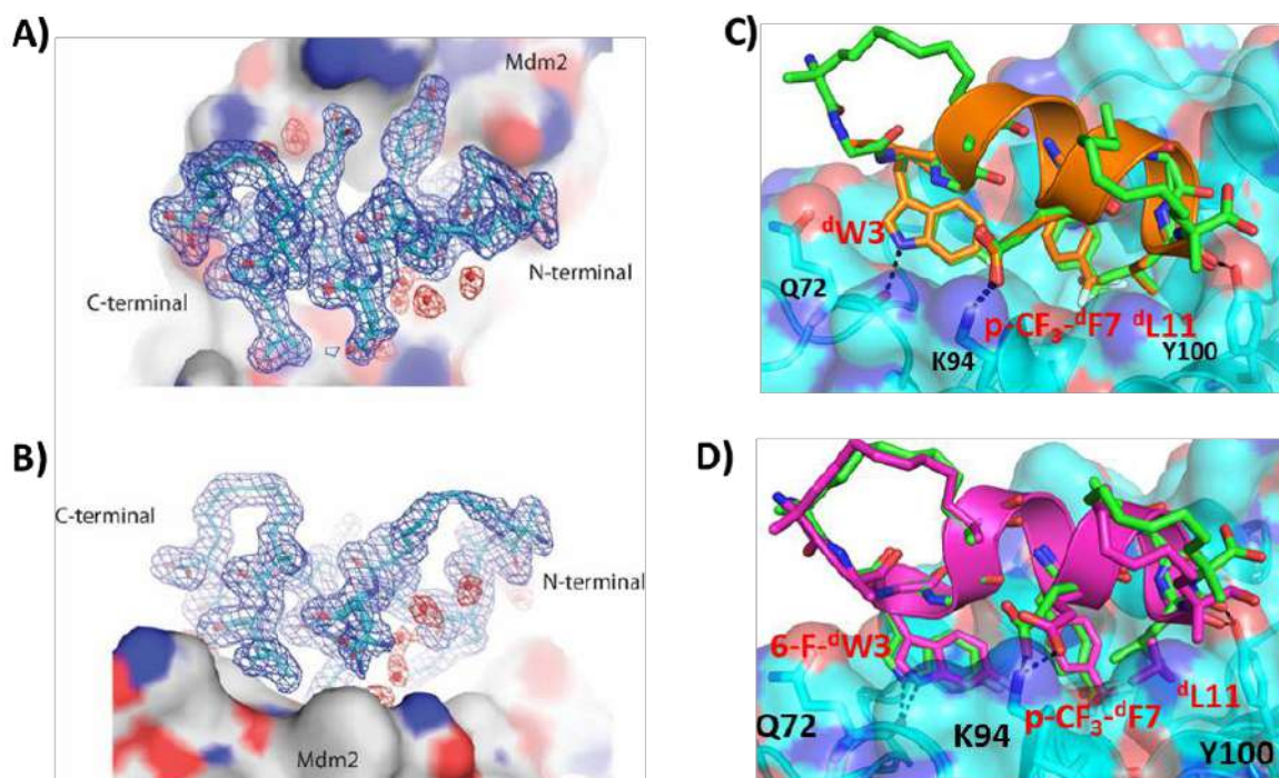
Figure 11: (A) Top down view of ^d\text{PMI-}\delta(1-5, 9-12) bound to Mdm2. (B) 90^\circ rotation of the ^d\text{PMI-}\delta(1-5, 9-12) -Mdm2 complex orientation shown in panel A), which clearly depicts the presence of both hydro-carbon staples in ^d\text{PMI-}\delta(1-5, 9-12) . The 2F_o - F_c map electron density map (shown with the blue mesh) for ^d\text{PMI-}\delta(1-5, 9-12) was contoured at 1.0\sigma . Interfacial structured waters involved in Mdm2- ^d\text{PMI-}\delta(1-5, 9-12) complex formation are shown using the red mesh. (C) Comparison of crystal structure of ^d\text{PMI-}\delta(1-5, 9-12) - Mdm2 complex with the ^d\text{PMI-}\delta - Mdm2 structure (PDB ID: 3TPX). The Mdm2 is shown as surface (cyan) with the bound ^d\text{PMI-}\delta(1-5, 9-12) (green) and ^d\text{PMI-}\delta (orange) peptides are shown as cartoon. The three critical residues ( ^d\text{W3} , p\text{-CF}_3\text{-}^d\text{F7} and ^d\text{L11} in ^d\text{PMI-}\delta , 6\text{-F-}^d\text{W3} , p\text{-CF}_3\text{-}^d\text{F7} and ^d\text{L11} in ^d\text{PMI-}\delta(1-5, 9-12) ) and residues involved in protein – peptide interactions are shown as sticks and the interactions are highlighted (black dashed lines). (D) Comparison of computationally modelled structure of ^d\text{PMI-}\delta(1-5, 9-12) - Mdm2 complex with the crystal structure of ^d\text{PMI-}\delta(1-5, 9-12) - Mdm2 complex. The Mdm2 is shown as surface (cyan) with the bound modelled ^d\text{PMI-}\delta(1-5, 9-12) (magenta) and experimental ^d\text{PMI-}\delta(1-5, 9-12) (green) peptides are shown as cartoon. The three critical residues ( 6\text{-F-}^d\text{W3} , p\text{-CF}_3\text{-}^d\text{F7} and ^d\text{L11} ) and residues involved in protein – peptide interactions are shown as sticks and the interactions are highlighted (black dashed lines).
