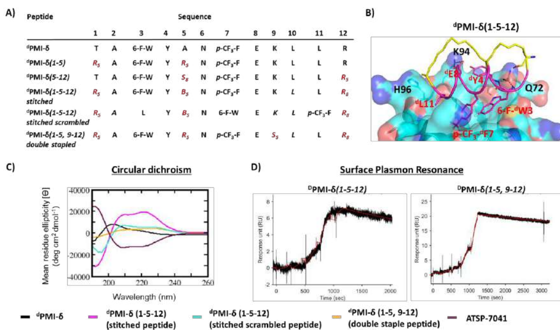
Figure 7: (A) Sequences of linear, stapled and stitched ^d\text{PMI-}\delta peptides are shown. (B) MD snapshot of stitched ^d\text{PMI-}\delta(1-5-12) -Mdm2 complex. Mdm2 is shown as surface and bound peptide (magenta) is shown as cartoon with interacting residues highlighted in sticks. The hydrocarbon stitch (linker) is highlighted in yellow. Hydrogen bond interactions are shown as dotted lines (black). (C) Secondary structure analysis of linear, double stapled, stitched ^d\text{PMI-}\delta and ATSP-7041 peptides determined through Circular dichroism (CD). Note that this CD spectra of linear, double stapled and stitched ^d\text{PMI-}\delta peptides is inverted, as expected for a peptide consisting of D-amino acids only. (D) Binding activity of double stapled and stitched ^d\text{PMI-}\delta peptides toward Mdm2 protein determined through SPR.
