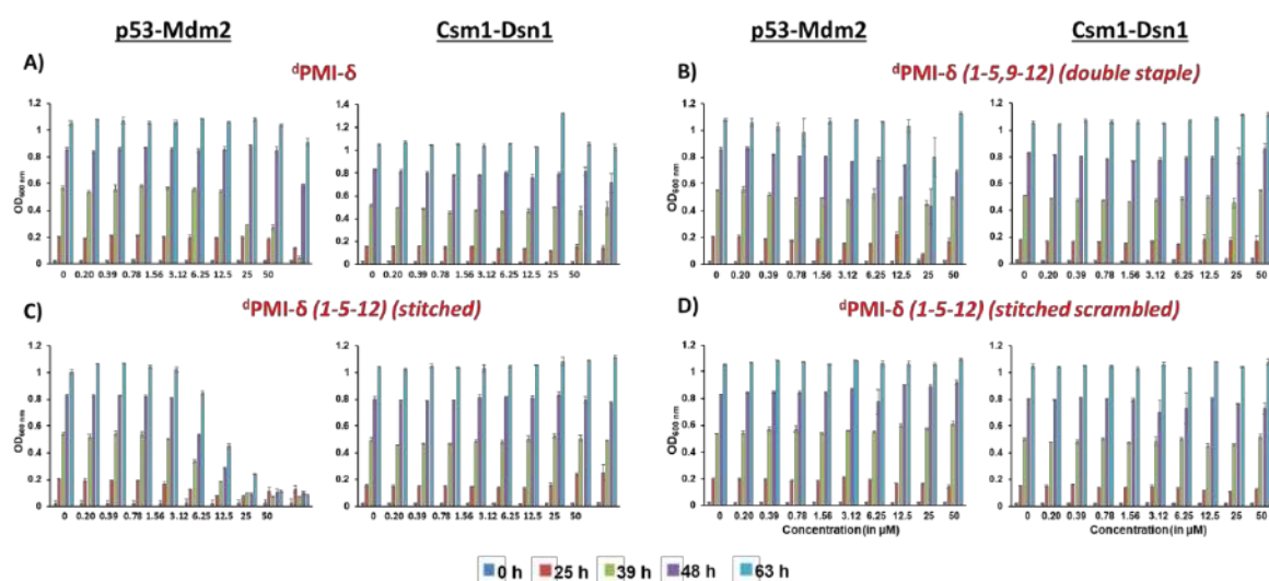
Figure 9: Overnight cultures of ABC9A strain containing plasmids encoding either Gal4 AD-p53 (1-52)/Gal4 BD-Mdm2 or Gal4 AD-Csm1/Gal4 BD-Dsn1 were inoculated at \text{OD}_{600}=0.2 into selective medium containing DMSO or ^d\text{PMI-}\delta or ^d\text{PMI-}\delta(1-5,9-12) , ^d\text{PMI-}\delta(1-5-12) and scrambled ^d\text{PMI-}\delta(1-5-12) peptides at the indicated concentrations in duplicate. For each strain, growth as measured by average \text{OD}_{600} of duplicate cultures is plotted at different time points following inoculation (0, 25, 39, 48, and 63 h). Ends of the vertical bar indicate the \text{OD}_{600} values of the duplicate cultures. Data for the ^d\text{PMI-}\delta , ^d\text{PMI-}\delta(1-5,9-12) , ^d\text{PMI-}\delta(1-5-12) and scrambled ^d\text{PMI-}\delta(1-5-12) peptides are shown in panels A, B, C and D respectively. For each peptide, data showing their effect on p53-Mdm2 and Csm1-Dsn1 interactions are presented on the left and right respectively.
