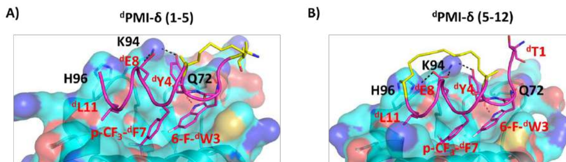
Figure 4: Structural representation of MD snapshot of (A) d PMI-δ(1-5)-Mdm2 and (B) d PMI-δ(5-12)-Mdm2 complex. Mdm2 is shown as surface and bound peptide is shown as cartoon with interacting residues highlighted in sticks. The hydrocarbon linker is highlighted in yellow. Hydrogen bond interactions are shown as dotted lines (black).
