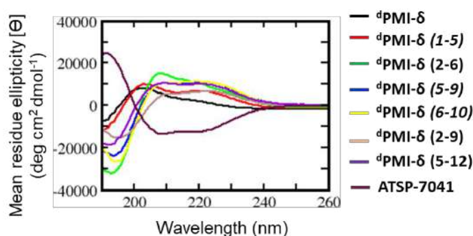
Figure 3: Secondary structure analysis of linear, stapled ^d\text{PMI-}\delta and ATSP-7041 peptides determined through Circular dichroism (CD). Note that this spectra of linear and stapled ^d\text{PMI-}\delta peptides are inverted, as expected for a peptide consisting of D-amino acids only.
