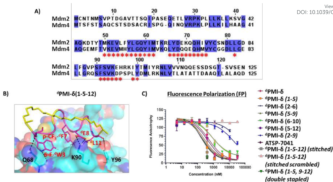
Figure 10: (A) Sequence comparison of N-terminal domains of Mdm2 and Mdm4. Identical residues are highlighted and binding pocket residues (residues that are within 6 Å of bound peptide) are highlighted as *. (B) MD snapshot of stitched d PMI-δ(1-5-12)-Mdm4 complex. Mdm4 is shown as surface and bound peptide is shown as cartoon with interacting residues highlighted as sticks. The hydrocarbon stitch (linker) is highlighted in yellow. Hydrogen bond interactions are shown as dotted lines (black). (C) Fluorescence polarization (FP) (0.001% Tween-20) binding analysis of linear, stapled, stitched d PMI-δ and ATSP-7041 peptides and Mdm4 protein.
