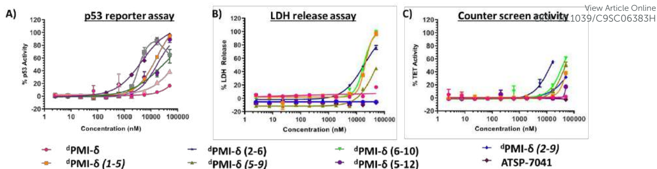
Figure 6: (A) Linear, stapled dPMI-\delta and ATSP-7041 peptides titrated on to HCT116 p53 reporter cells and p53 transcriptional activation assessed in the presence of 2% of serum. (B) Linear, stapled dPMI-\delta and ATSP-7041 peptides titrated on to HCT116 cells and LDH release measured. (C) Activity of linear, stapled dPMI-\delta and ATSP-7041 peptides measured in a counter screen.
