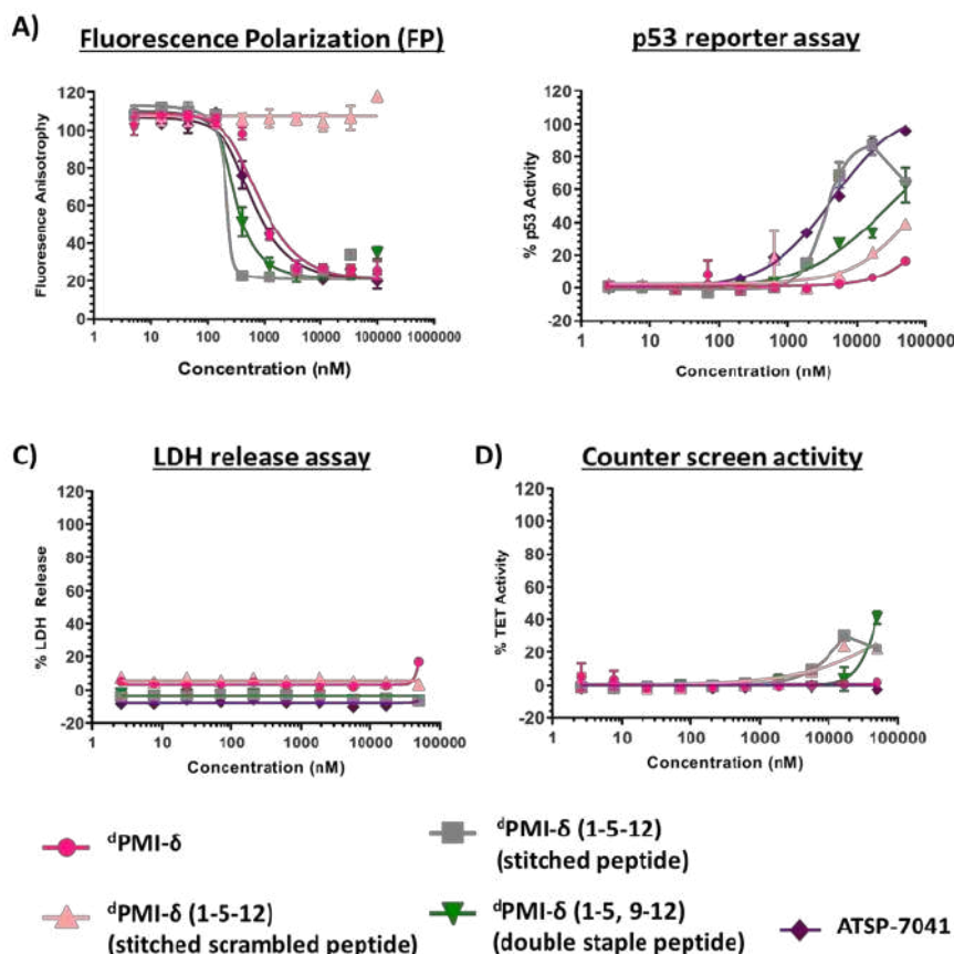
Figure 8: Binding activity of linear, double stapled, stitched dPMI-\delta and ATSP-7041 peptides toward Mdm2 protein determined through (A) Fluorescence polarization (FP) (0.001% Tween-20) assay. (B) Linear, double stapled, stitched dPMI-\delta and ATSP-7041 peptides were titrated on to HCT116 p53 reporter cells and p53 transcriptional activation assessed in the presence of 2% serum. (C) Linear, double stapled, stitched dPMI-\delta and ATSP-7041 peptides were titrated on to HCT116 cells and LDH release measured. (D) Activity of linear, double stapled, stitched dPMI-\delta and ATSP-7041 peptides were measured in a counter screen.
