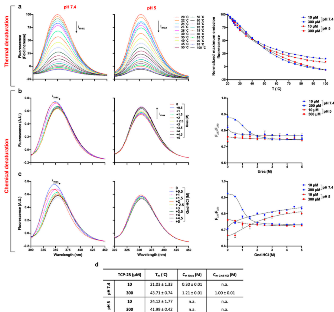
Figure 3. Thermal and chemical denaturation of TCP-25. TCP-25 (10 and 300 \mu\text{M} ) in 10 mM Tris at pH 7.4 or in 10 mM NaOAc at pH 5.0 was denatured by increasing temperature (a) or by addition of increasing amounts of urea (b) or Gdn-HCl (c). The unfolding process was analyzed by recording the emission spectra between 300 and 450 nm upon excitation at 280 nm. Representative emission spectra are shown for 300 \mu\text{M} TCP-25 dissolved at pH 7.4 or 5.0 with different denaturing methods ( n = 3 ). On the right, the denaturation curves are reported. In the case of thermal denaturation, data were obtained by fitting the normalized maximum emission fluorescence as a function of the temperature. For the chemical denaturation, results were obtained using the fluorescence ratio ( F_{337}/F_{350} ) as a function of the concentration of the chemical agent. Each data point represents the mean \pm SEM ( n = 3 ). (d) Table showing T_m and C_m \pm SEM calculated from the denaturation curves obtained from 3 independent experiments done in duplicate ( n = 3 ). \rightarrow indicates shift in the maximum fluorescence intensity ( \lambda_{\max} ); \uparrow I_{\max} and \downarrow I_{\max} indicate increase and decrease in maximum fluorescence intensity, respectively.
