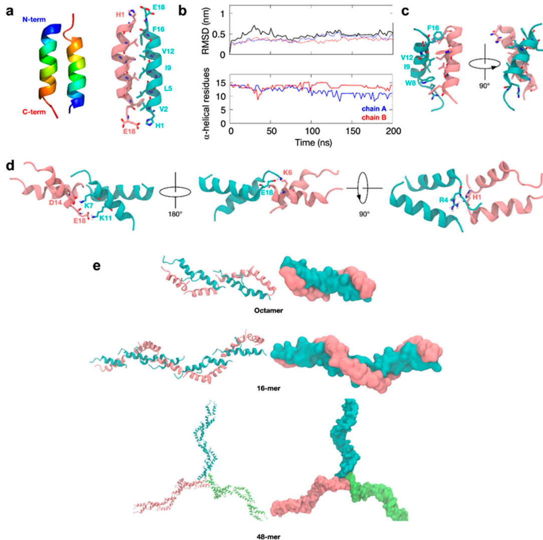
Figure 6. HVF18 idealized helix oligomerization. (a) A homology model of HVF18 was built as an ideal alpha-helical structure and the ClusPro program was used to generate a dimer. Two docking simulations were performed, and representative structures from the most populated clusters were aligned and colored in rainbow (left). Residues forming the dimer interface are highlighted in stick representation (right). (b) A 200-ns MD simulation was then performed, and the backbone root-mean-square deviation (RMSD) representing the structural drift during the simulation (top) was calculated for individual subunits (thin blue and red lines) and for the overall dimer (thick black line). The secondary structure preservation plot (bottom) shows the number of residues remaining in an alpha-helical conformation throughout the simulation for each chain. (c) Final image of the simulation showing residues that form the dimeric interface in stick representation. (d) Using the final snapshot as input for ClusPro, the structure of a tetramer was built. The representative structure of the most populated cluster is shown with the tetrameric interface highlighted in stick representation. (e) Octamer, 16-mer, and 48-mer structures were subsequently built using common oligomerization interfaces.
