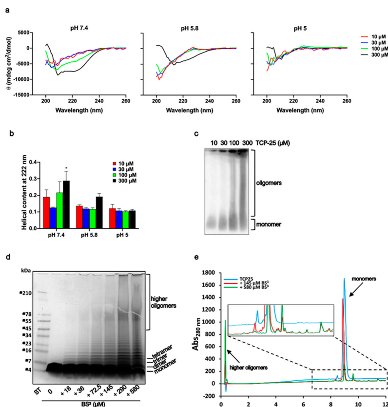
Figure 2. Structural analyses of TCP-25 oligomers. (a) Representative far-UV CD spectra of TCP-25 dissolved at 10, 30, 100 and 300 \mu M in 10 mM Tris at pH 7.4 or in 10 mM NaOAc at pH 5.8 and 5.0. All the spectra were acquired at 25 ^{\circ} C. The change in secondary structure was affected by pH and TCP-25 concentration ( n = 3 ). (b) \alpha -helical content \pm SD calculated from CD spectra obtained at 222 nm. A significant increase in \alpha -helical content was observed for 300 \mu M TCP-25 in 10 mM Tris at pH 7.4. * indicates p < 0.05 using one-way ANOVA with Dunnett's multiple comparison test ( n = 3 ). (c) Separation on 4–16% ( w/v ) BN-PAGE followed by western blot analysis shows an increased oligomerization of TCP-25 at higher concentrations. One representative image of 3 independent experiments is shown ( n = 3 ). (d) TCP-25 was cross-linked with different concentration of BS 3 for 30 min and then analyzed on 16.5% Tris-Tricine gel followed by Coomassie staining. Increased concentration of crosslinker yielded TCP-25 oligomers of higher molecular weights. One representative image of 3 independent experiments is shown ( n = 3 ). (e) Reverse-phase C18 chromatography of TCP-25 in the absence (blue line) or in the presence of 145 \mu M (red line) or 540 \mu M (green line) BS 3 showing an alteration in the elution profiles.
