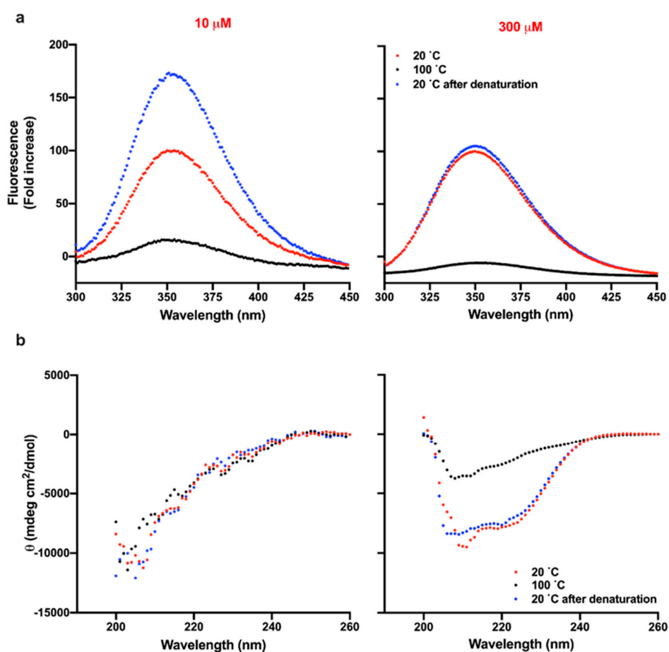
Figure 4. Reversibility of thermal denaturation of TCP-25 at pH 7.4. 10 and 300 \mu M TCP-25 in 10 mM Tris at pH 7.4 were denatured by exposing the peptide to 100 °C and bringing the temperature back to 20 °C. The re-folding was analyzed by recording the intrinsic fluorescence of the peptide (a) or secondary structure (b). The spectra were collected at 20 (red), 100 (black), and 20 °C after denaturation at 100 °C (blue). Each graph is a representative result of 3 independent experiments ( n = 3 ).
