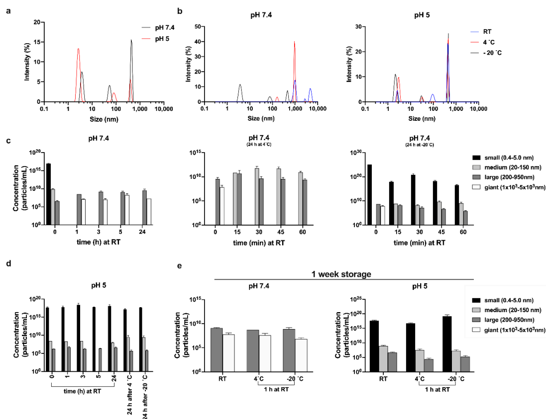
Figure 5. Size of oligomers and their distribution. (a,b) Representative size distribution by intensity of 300 \mu M TCP-25 in 10 mM Tris at pH 7.4 or in 10 mM NaOAc at pH 5.0. Sizes of oligomers at pH 7.4 (c,e) and pH 5.0 (d,e), and their distributions after storage at RT, 4, or -20 °C for up to 24 h (c,d) or after 1 week of storage (e). Oligomers were classified into 4 families: small (0.4–5 nm, black bars), medium (20–150 nm, light gray bars), large (200–950 nm, dark gray bars), and giant ( 1 \times 10^3 – 5 \times 10^3 nm, white bars). For each sample, spectra were recorded three times with 11 sub-runs using the multimodal mode. In the graphs, the concentrations of the oligomers belonging to different families are reported as the average \pm SD ( n = 2 ).
