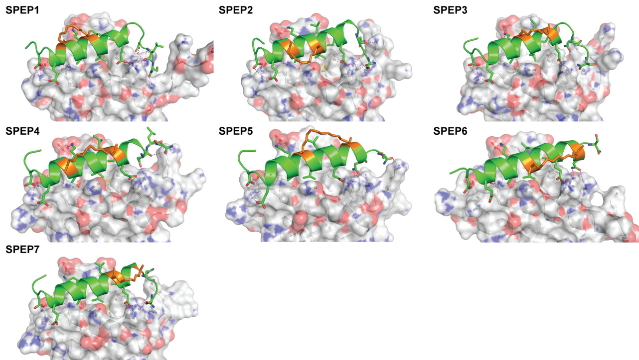
Fig. 5 Structural representations of MD snapshots of \text{DHB}_{\text{DAXX}} /SPEP complexes. Structural models for \text{DHB}_{\text{DAXX}} complexes with SPEP1, SPEP2, SPEP3, SPEP4, SPEP5, SPEP6 and SPEP7 are shown. The \text{DHB}_{\text{DAXX}} (white) and bound peptide (green) conformations are shown as surface and cartoon representations, respectively with interacting residues and staples (orange) highlighted in sticks. Hydrogen bonds are indicated by dotted lines (magenta).
